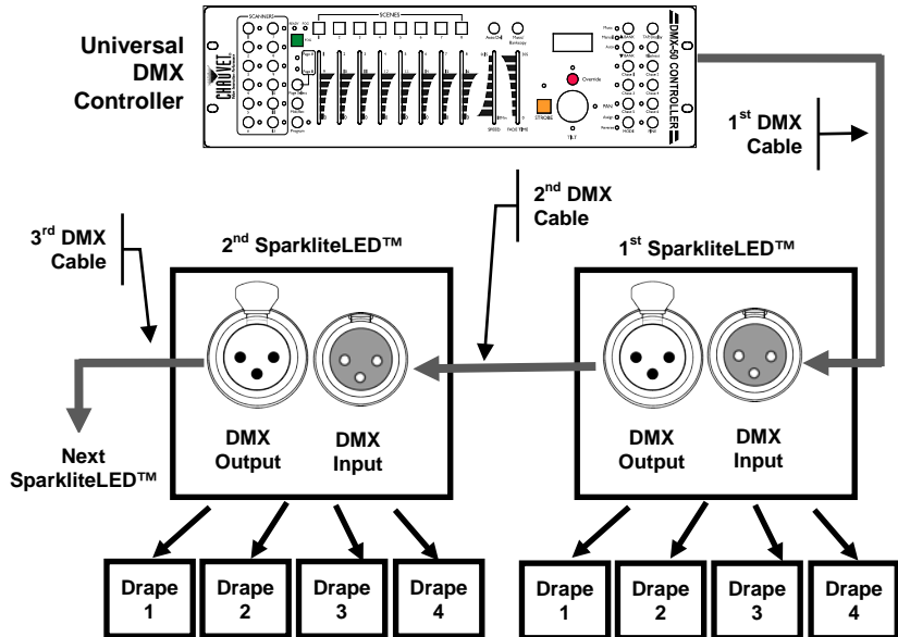
DMX Data Connection Diagram
